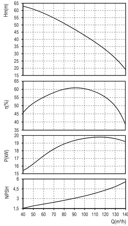
SD430B 25HP (2900 d/d - rpm)
