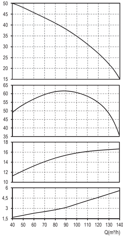
SD430B 20HP (2900 d/d - rpm)
