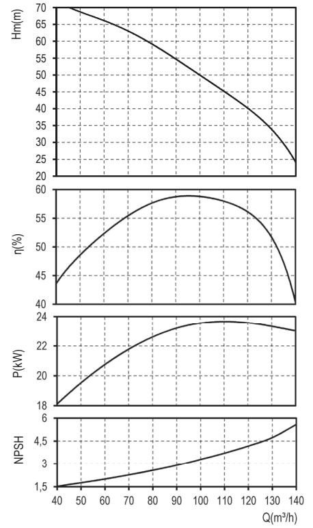
SD430B 30HP (2900 d/d - rpm)
