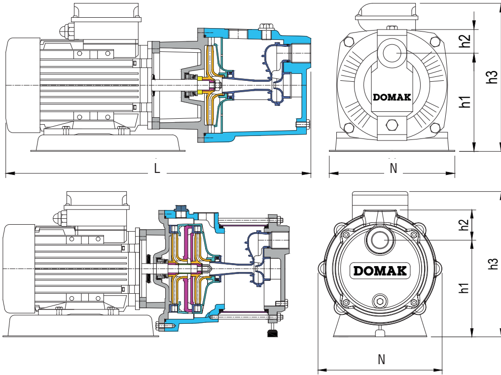
JET 1HP - 1,5HP - 3HP (2900 d/d - rpm)
